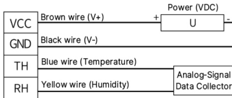
Analog Wiring Schematic Diagram
